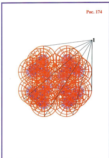
Fig. 174. Fourth-order superspaces.
