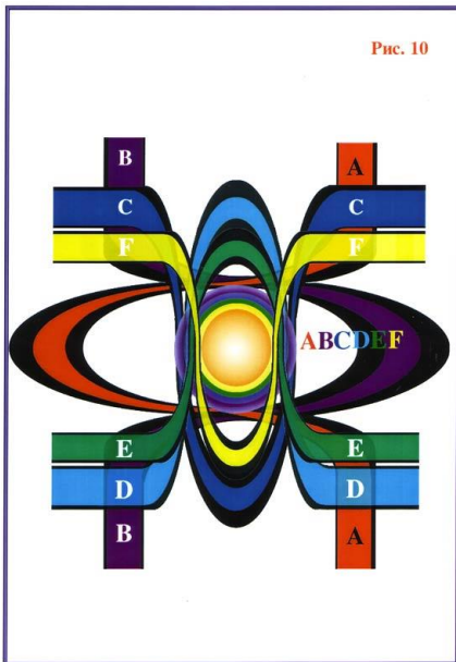
Fig. 10. The Mergence of Six Primary Matters A, B, C, D, E, F in the zone of space curvature with the formation of hybrid ABCDEF .
