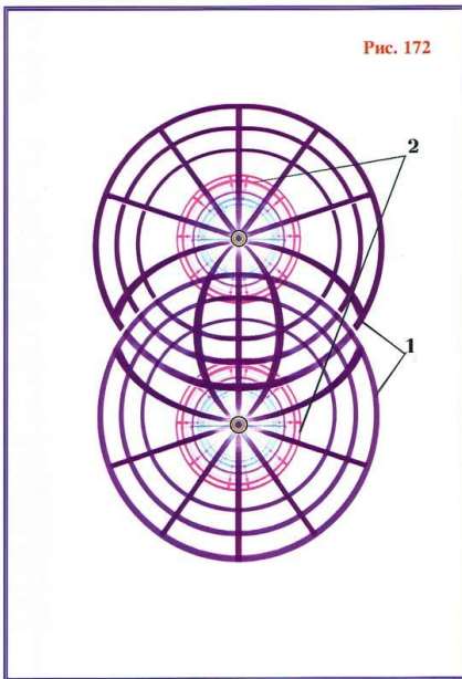
Fig. 172. Second-order superspaces.
