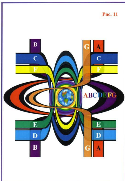
Fig. 11. The Merger of Seven Primary Matters A, B, C, D, E, F, G in a zone of space curvature leading to formation of hybrid ABCDEFG .
