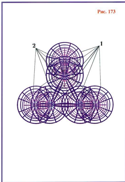
Fig. 173. Third-order superspaces.
